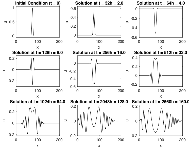
Fig. 6.6: Various timestep solutions for Sine-Gordon using DPSM based on equation 6.2.
