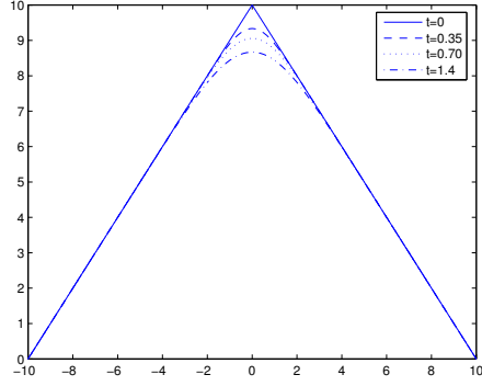
Fig. 6.2: Degree 4 iterate for solving u_t = u_{xx} using a centered difference scheme.
